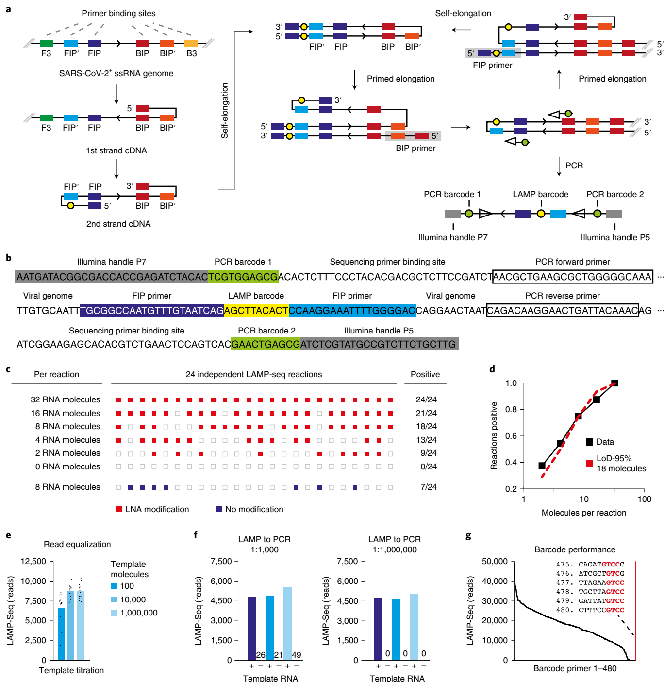
Fig. 1 | LAMP-Seq: a scalable deep sequencing-based approach for SARS-CoV-2 detection. a , Schematic of anticipated enzymatic reactions and reaction products. b , Annotated amplicon sequence for Illumina NGS of SARS-CoV-2 RT-LAMP products. c , Sensitivity assessment of LAMP-Seq using 24 reactions per condition, templated with the indicated numbers of RNA molecules per reaction. Filled squares indicate barcodes with read numbers >10% of median calculated from 24 positive samples. LNA modifications increase melting temperature from 53.7 °C to 60.1 °C for F3 and from 50.0 °C to 57.3 °C for B3. d , Estimation of the LoD-95 based on probit analysis of the fraction of positives among 24 replicates. e , LAMP-Seq reactions templated with 100, 10,000 or 100,000 RNA molecules. Reactions were PCR amplified and sequenced on an Illumina MiSeq sequencer. Absolute read counts per sample are shown from ten experimental replicates per condition. f , Quantitative assessment of barcode swapping in LAMP-Seq and dependence on pre-dilution of pooled RT-LAMP reactions before PCR (left panel, 1,000-fold; right panel, 1,000,000-fold). LAMP-Seq was performed as described in the Methods section, with the exception that synthetic RNA was used as the template instead of a swab sample, no Bst 3.0 or Tris buffer was added, and no LNA-modified primers were used. Numbers in the plot indicate read numbers for non-templated negative control reactions. g , Empirical performance assessment of 480 randomly chosen LAMP-Seq barcode primers. The barcoded FIPs were mixed at an equimolar concentration and used as a pool in four replicate LAMP-Seq reactions templated by RNA. Raw sequencing data were analyzed using LAMP-Seq Inspector v1.0 ( http://manuscript.lamp-seq.org/Inspector.htm ). Read counts are shown for barcodes in descending order. The six worst-performing barcode sequences are highlighted in red, and the respective sequences are provided in the inset. ssRNA, single-stranded RNA.
